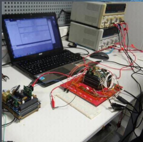
Software Test
